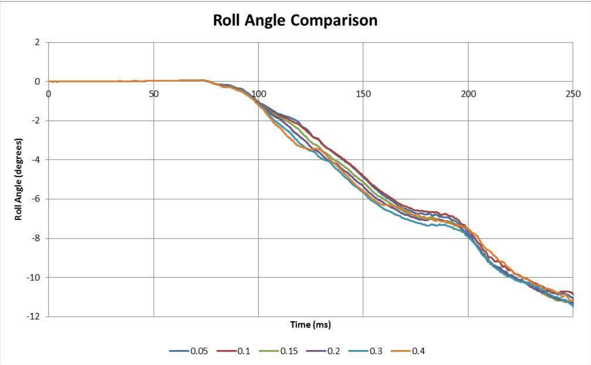
b. Vehicle Roll Motion Prior to Rear Wheel Impact with Barrier
