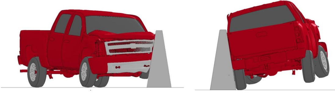
Figure 64. Maximum ZOI Positions for the Model with Lower Control Arm and Steering Link Failures
