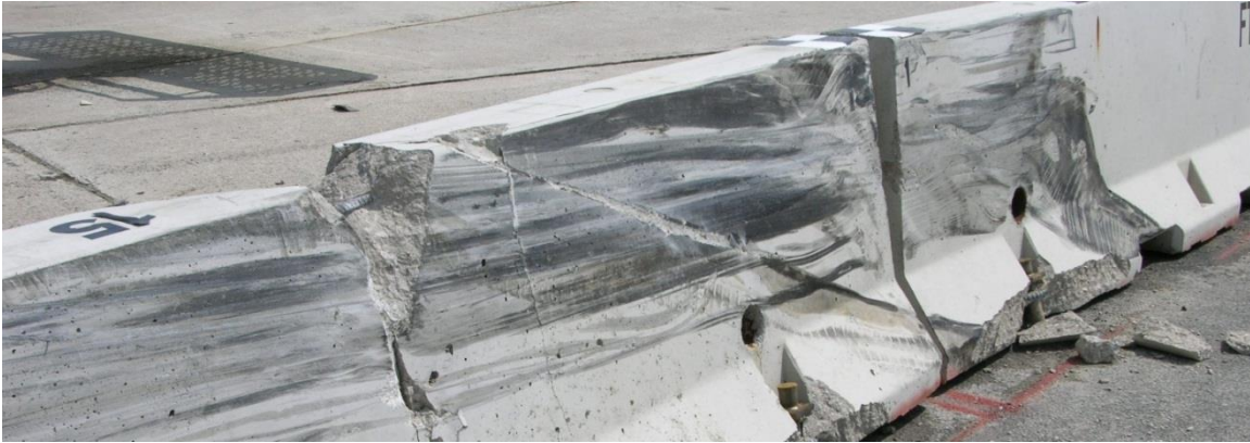
b. Contact Marks from Test No. FTB-2
