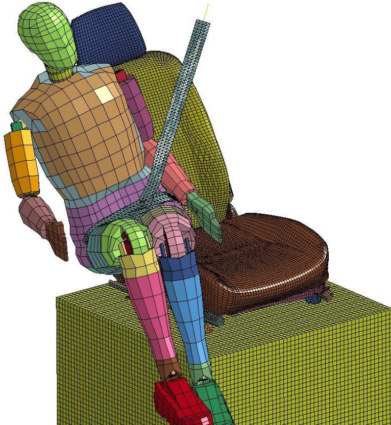
Figure 77. Seatbelt Stretch
