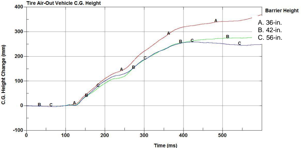
Figure 61. Tire Deflation Simulation Vehicle C.G. Height
