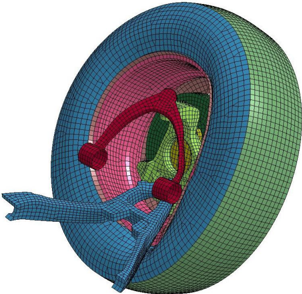
Figure 57. Suspension Damage for the Model with Tire Deflation
