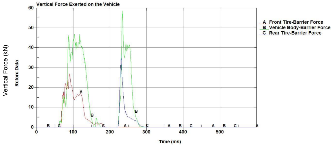
Figure 50. Contact Forces by Component
