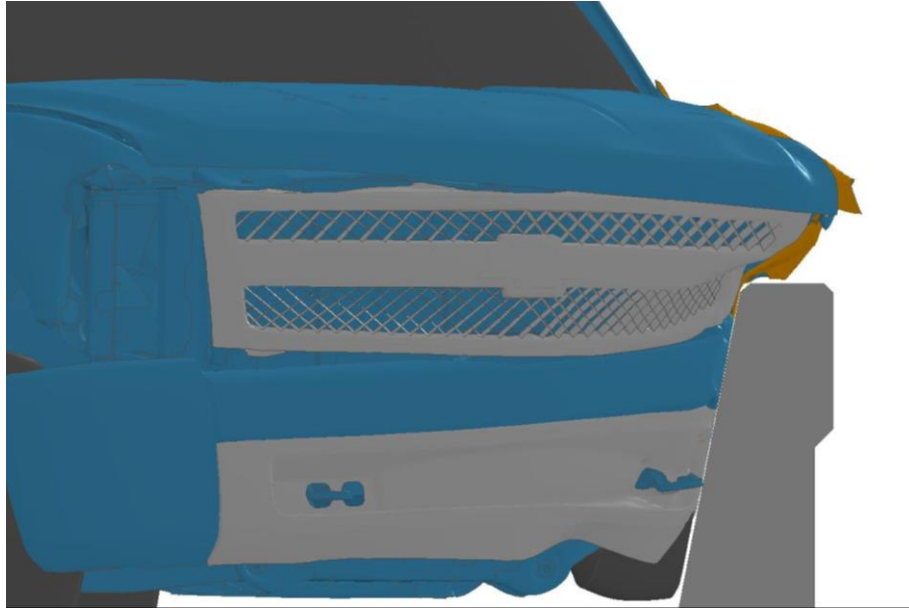
Figure 33. Fender Protrusion Over the Barrier (Note: Fender is orange for distinction)
