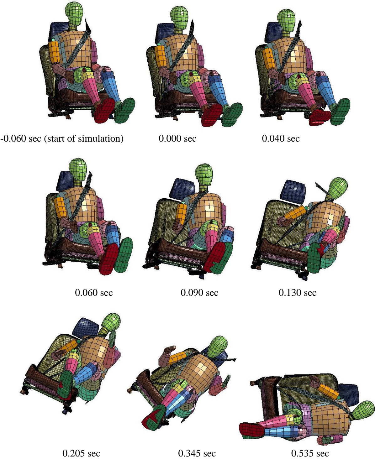
Figure 81. Dummy Reaction in the Vehicle
