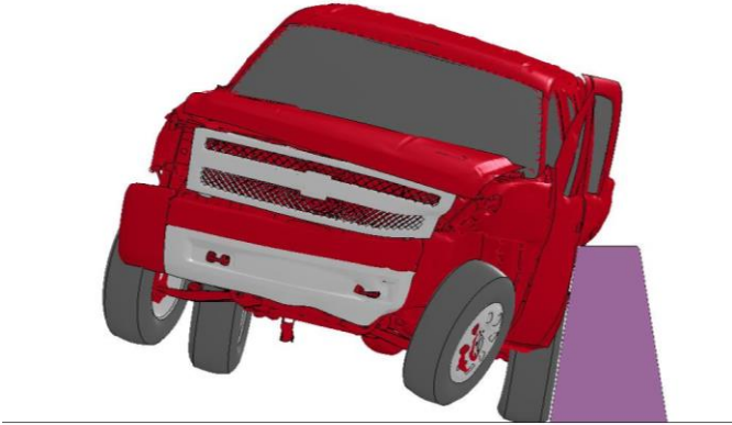
Figure 52. Vehicle Roll Toward the Barrier
