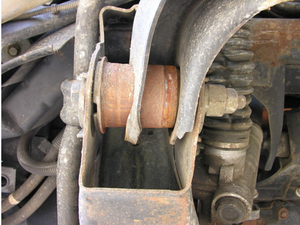
Front Connection Slip (View looking toward longitudinal centerline of vehicle)
