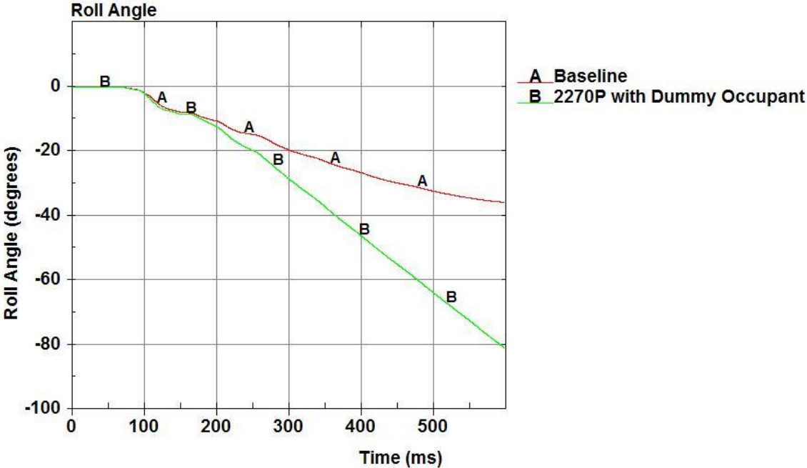
Figure 88. Vehicle Roll Angle
