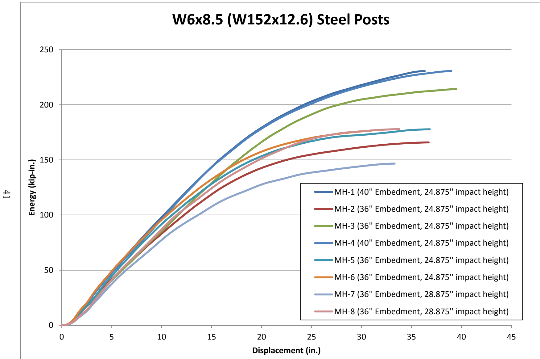
Figure 24. Energy vs. Displacement Plots, 36 in. Embedment and 28.875 in. Load Height
